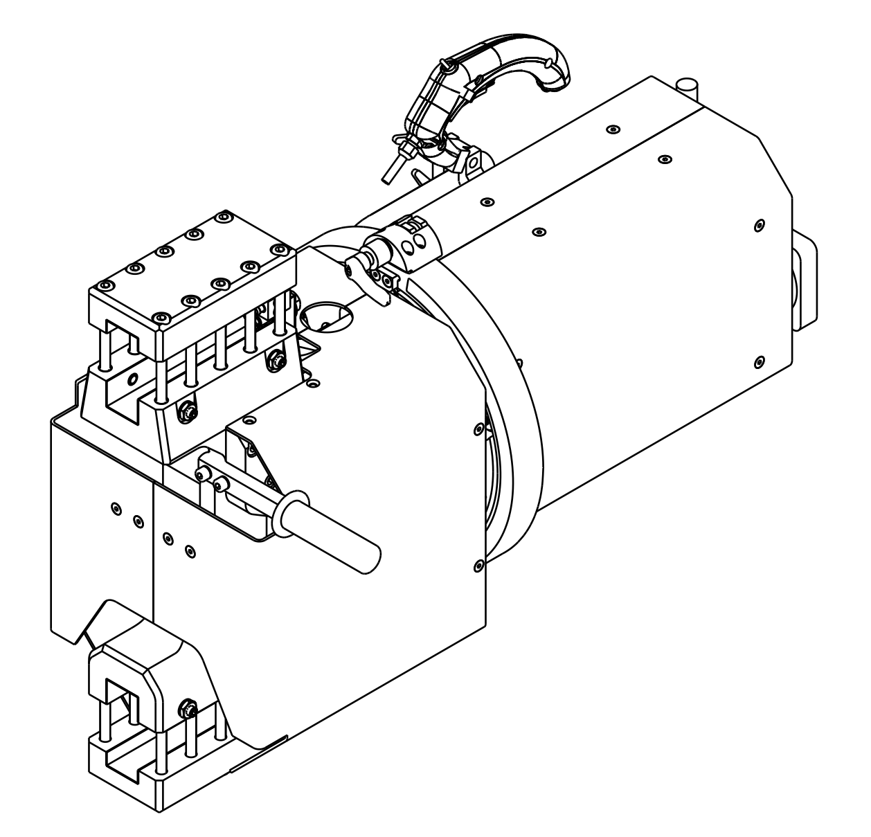
Transformer integrated X welding gun
